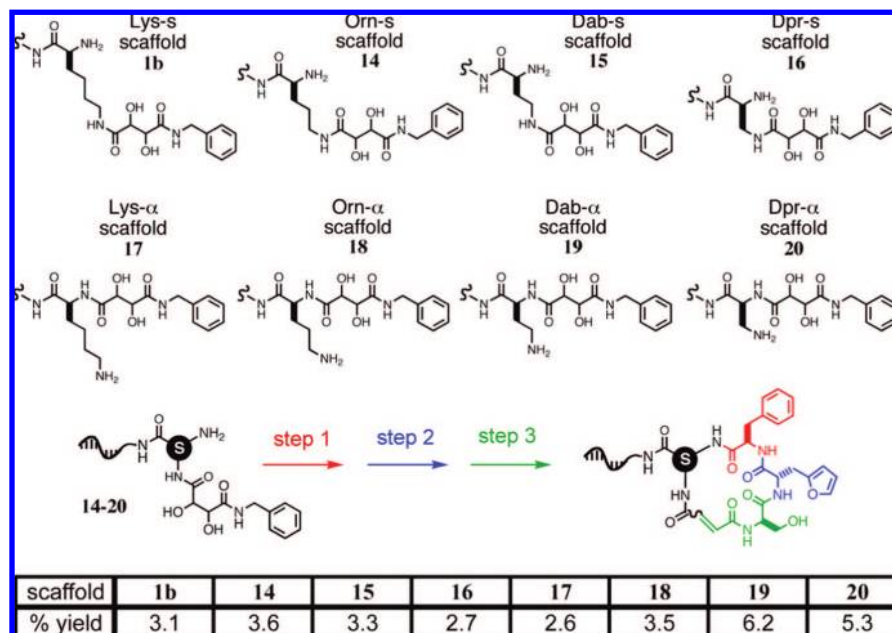
Figure 8. Eight scaffolds for DNA-templated macrocycle syntheses. The tartaramide group (aldehyde precursor) can be placed on either the \alpha -amine or side-chain (“s”) amine, resulting in two different orientations of building blocks within the resulting macrocycles. The eight scaffolds (denoted by the circled S) were transformed into their corresponding macrocycles using the same reagents used in the synthesis of macrocycle 8b from scaffold 1b ; the respective overall percent yields for final purified macrocycles are shown in the table above.
