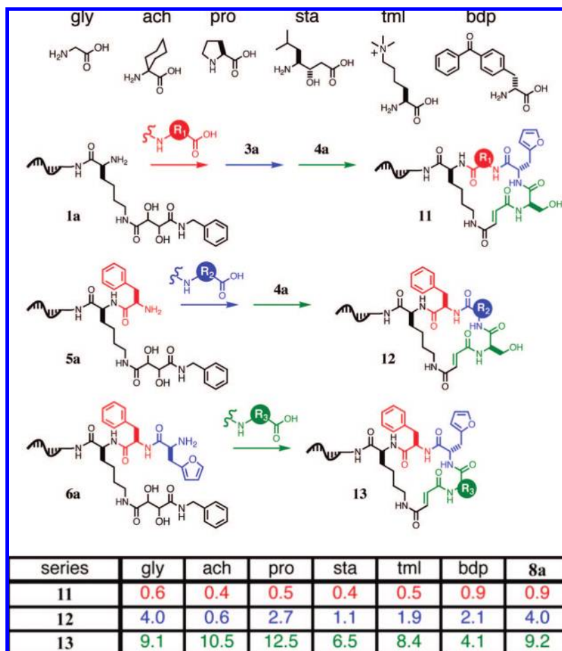
Figure 7. Systematic study of building-block compatibility with DNA-templated macrocycle synthesis. Using macrocycle 8a as a benchmark of “normal” reactivity, we selected a set of six distinct amino acids for substitution, one at a time, into the macrocycle at each of the three building block positions ( R_1 , R_2 , and R_3 ). Macrocycle series 11 (substitution at R_1 ), 12 (substitution at R_2 ), and 13 (substitution at R_3 ) were synthesized using the corresponding reagent sets and starting materials 1a , 5a , and 6a , respectively. Percent yields of each macrocycle as analyzed by PAGE using internal standards are shown in the table.
