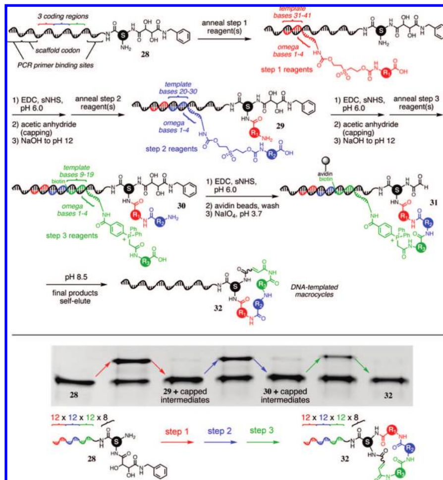
Figure 14. Synthesis of a 13 824-membered macrocycle library ( 32 ) from DNA template library 28 . Eight template library-linked scaffolds were processed in a single solution through three DNA-templated reactions, each using 12 building blocks each, to produce a final macrocycle library with 13 824 members. The synthesis was performed in triplicate, with an average overall purified yield of 1.6% as determined by PAGE (one example is shown in the gel above). In total, >375 pmol of library was produced, sufficient material for hundreds of in vitro selections.
