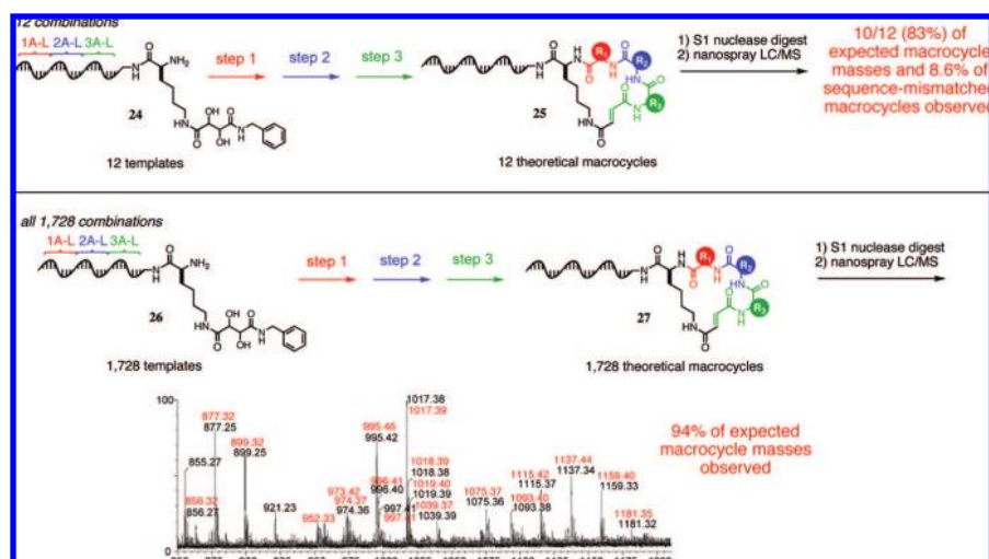
Figure 13. High-resolution LC/MS analysis of the 12-membered ( 25 ) and 1728-membered ( 27 ) DNA-templated macrocycle sublibraries. From library 25 , a stringent test of sequence specificity, 10 of 12 expected macrocycle masses were detected, and only 8.6% of masses corresponding to sequence-mismatched products were observed. For library 27 , 94% of expected masses were observed. The macrocycles eluted over a total of \sim 2400 s; the representative mass spectrum shown here is of a 35-s elution window. Expected masses are in red and observed masses are in black.
