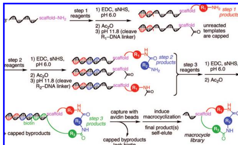
Figure 2. Capping-based strategy for DNA-templated macrocycle synthesis. The use of a capping reagent (here, acetic anhydride) prevents unreacted or improperly reacted material from participating in further reactions. The final streptavidin bead capture and macrocyclization steps achieve effective purification of the final product, obviating the need to purify after each DNA-templated reaction as in Figure 1 and reducing the total number of required manipulations.
