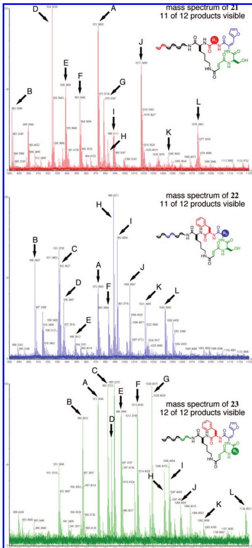
Figure 12. LC/MS analysis of 12-membered macrocycle libraries 21 , 22 , and 23 following S1 nuclease digestion. In total, 34 of the 36 expected macrocyclic species (94%) are visible.
